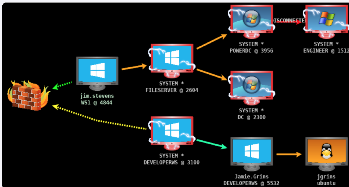
3: Client "graph view" of chained BEACONS ( source )
