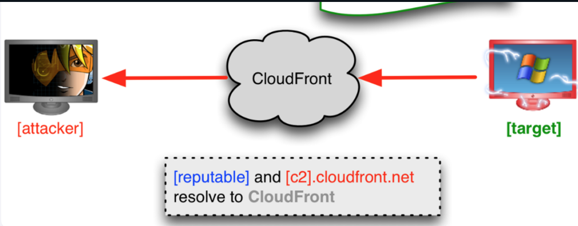
Figure 2: Domain fronted C2 connection ( source )
